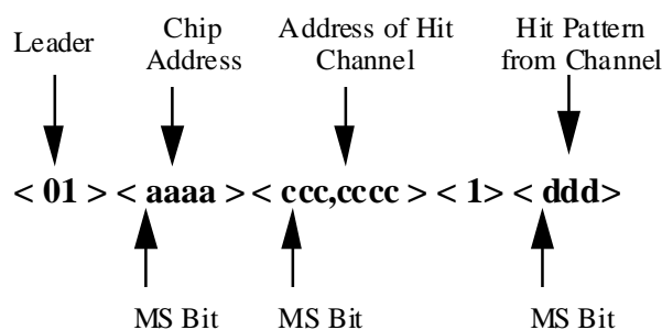
Figure 3.17b. Isolated hit data packet.
