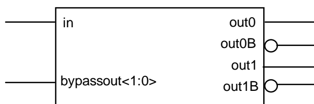
Figure 3.16. Token and Data Outputs circuit
