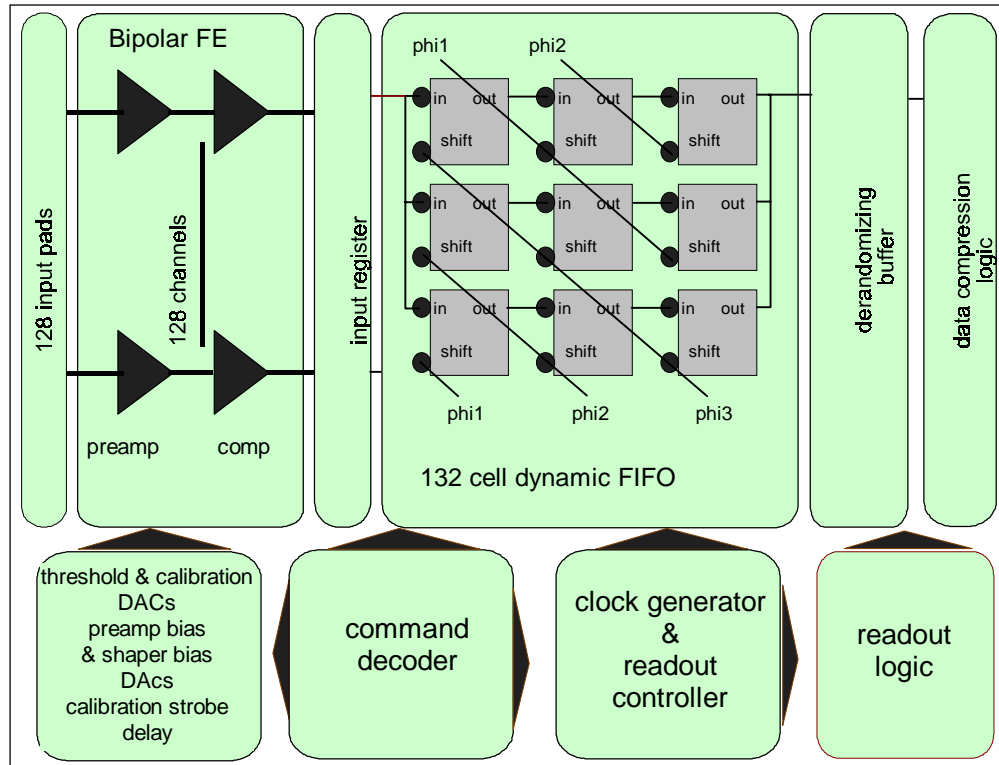
Figure 3.1. Block diagram of the ABCD chip.
